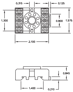
CR420KA2 Socket
