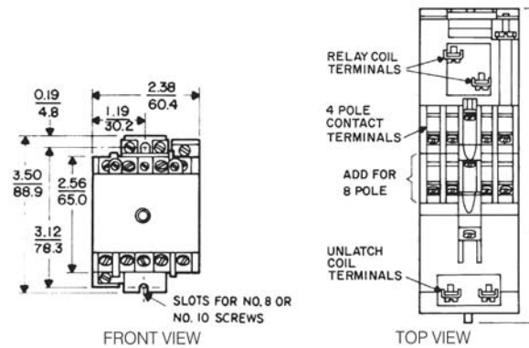
CR120BL AC Operated Latched Relay
