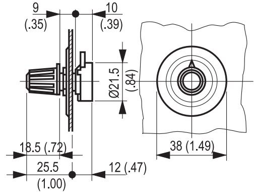
Remote Potentiometer
