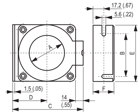
Differential Transformers
