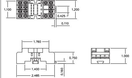
CR420MA Socket
