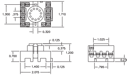
CR420KA3 Socket
